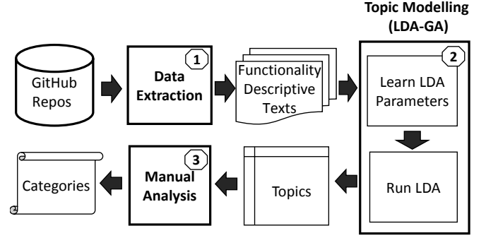
Figure 1: Overall Framework
